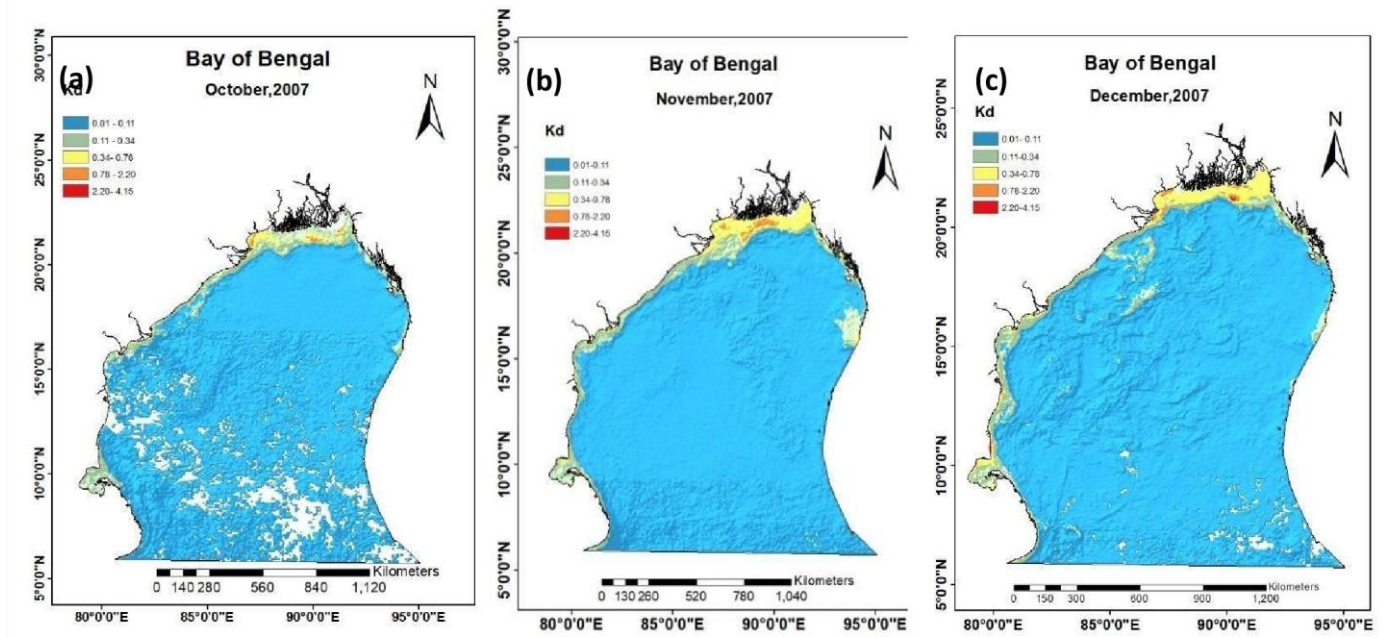
Figure 7: Composite image of Kd (a)pre-month; October, (b) affected-month; November, (c)post-month; December.
