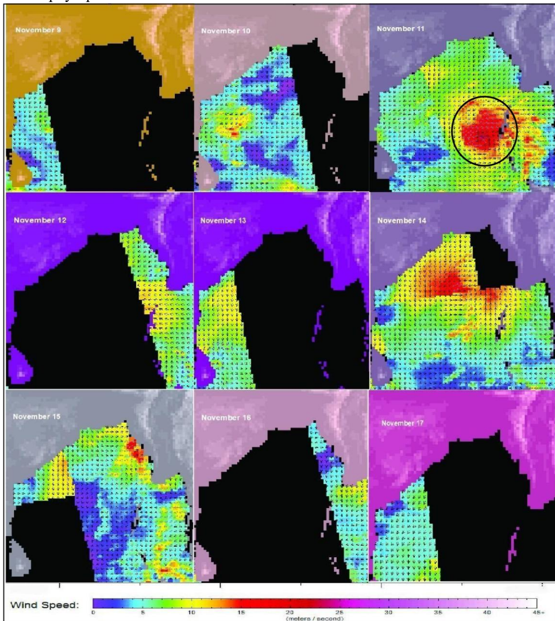
Figure 4: 'Quickcat scatterometer' derived wind speed and wind vector maps during 9 November, 2007 to 17 November, 2007 over
