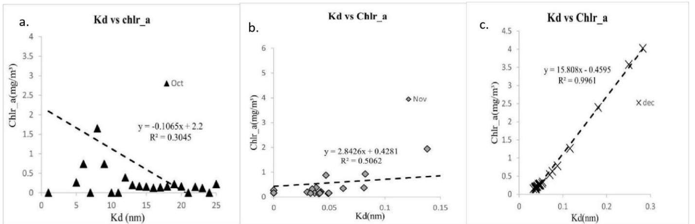
Figure 8: For Kd-Chlr_a The co-efficient of determination ( R^2 ) increases gradually from 0.3045 to 0.9961 due to the cyclone that is close to 1 (a,b,c)
