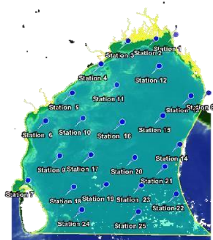
Figure 2: Elected tracking point of 25 stations for each month Chl_a,SST and Kd
